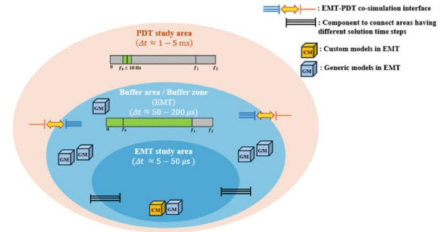
PDT-EMT co-simulation
