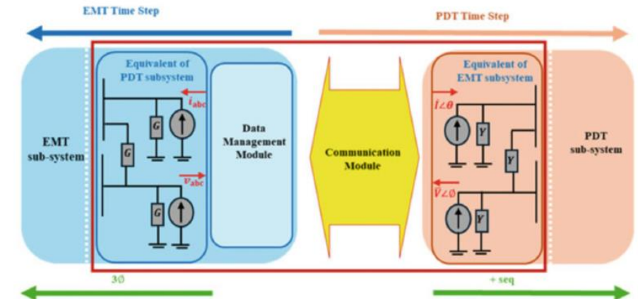
Info exchange between PDT and EMT domain
