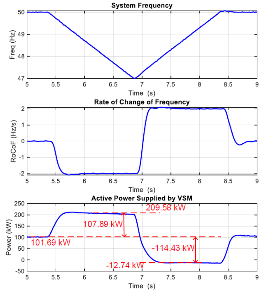
Diagram from “Great Britain Grid Forming Best Practice Guide”, 2023.
